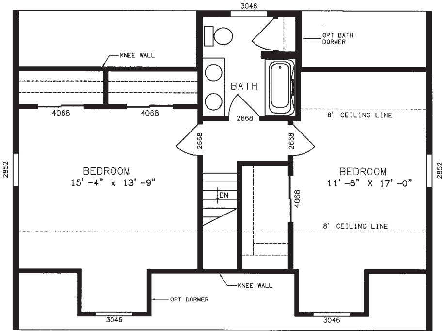
PLAN NO. VC3861 PROPOSED SECOND FLOOR (BY OTHERS) 17'0" X 40'0"
