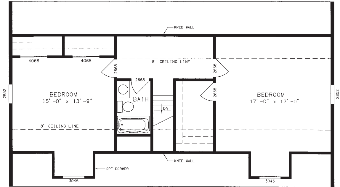
PLAN NO. VC3867 PROPOSED SECOND FLOOR (BY OTHERS) 17'0" X 48'0"
