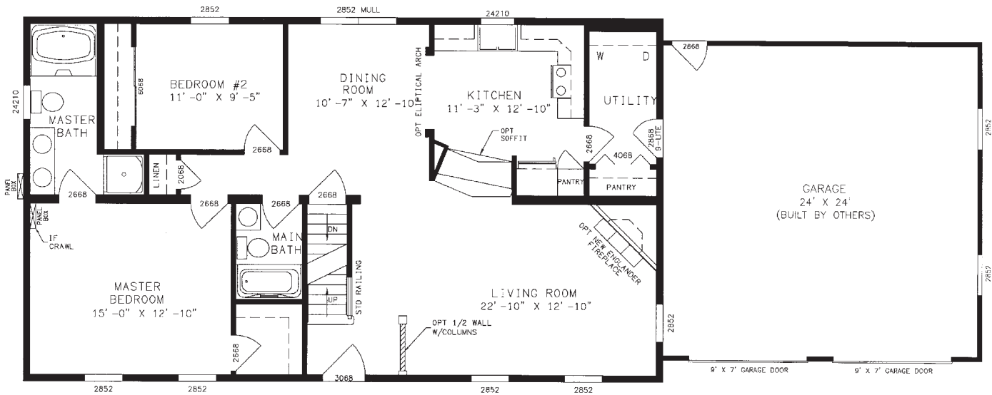
PLAN NO. VC3867 27'4" X 48'0" 1312 sq. ft.
