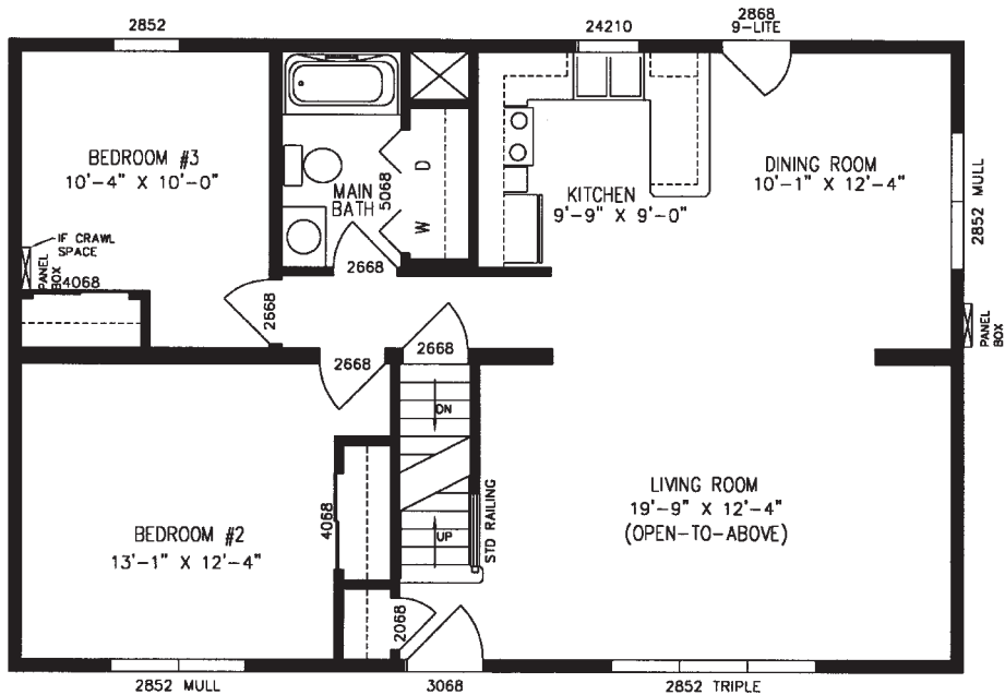
PLAN NO. PT5010 FIRST FLOOR 26'4" X 40'0" 2106 sq. ft.
