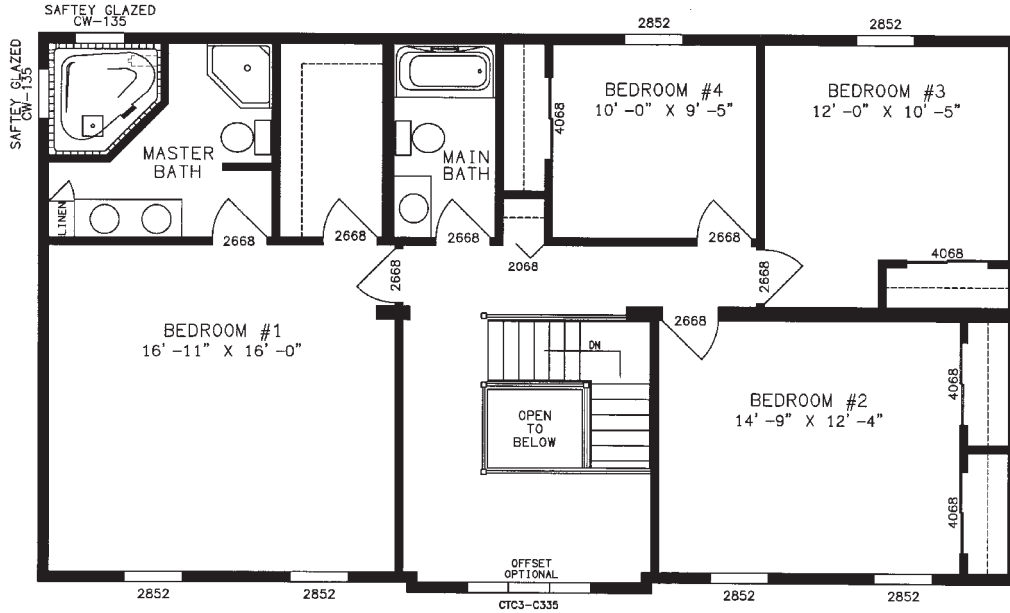
PLAN NO. PT5736 SECOND FLOOR 27'4" X 48'0"
